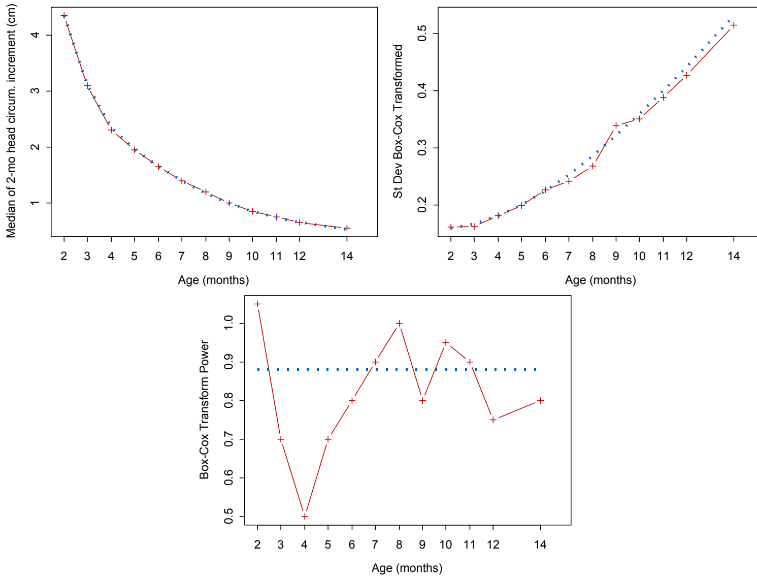
Figure A5.7 Fitting of the \mu , \sigma , and \nu curves of selected model for 2-month head circumference velocity for girls
