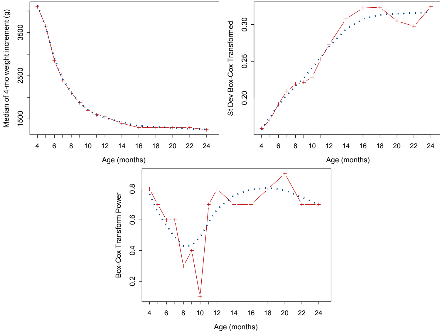
Figure A3.28 Fitting of the \mu , \sigma , and \nu curves of selected model for 4-month weight velocity for boys
