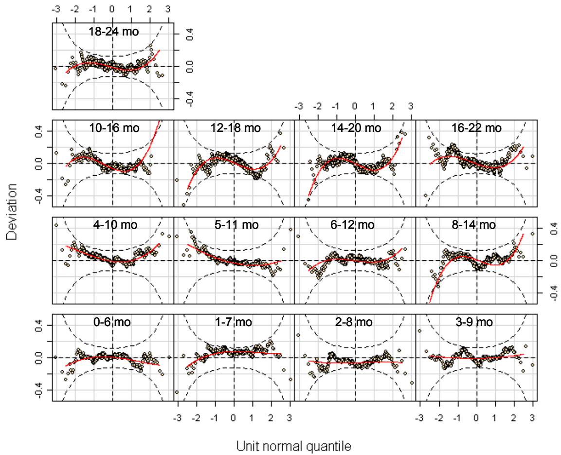
Figure A3.37 Worm plots from selected model [BCPE( \chi = \text{age}^{0.05} , df(\mu) = 10 , df(\sigma) = 5 , df(\nu) = 3 , \tau = 2 )] for 6-month weight velocity for boys
