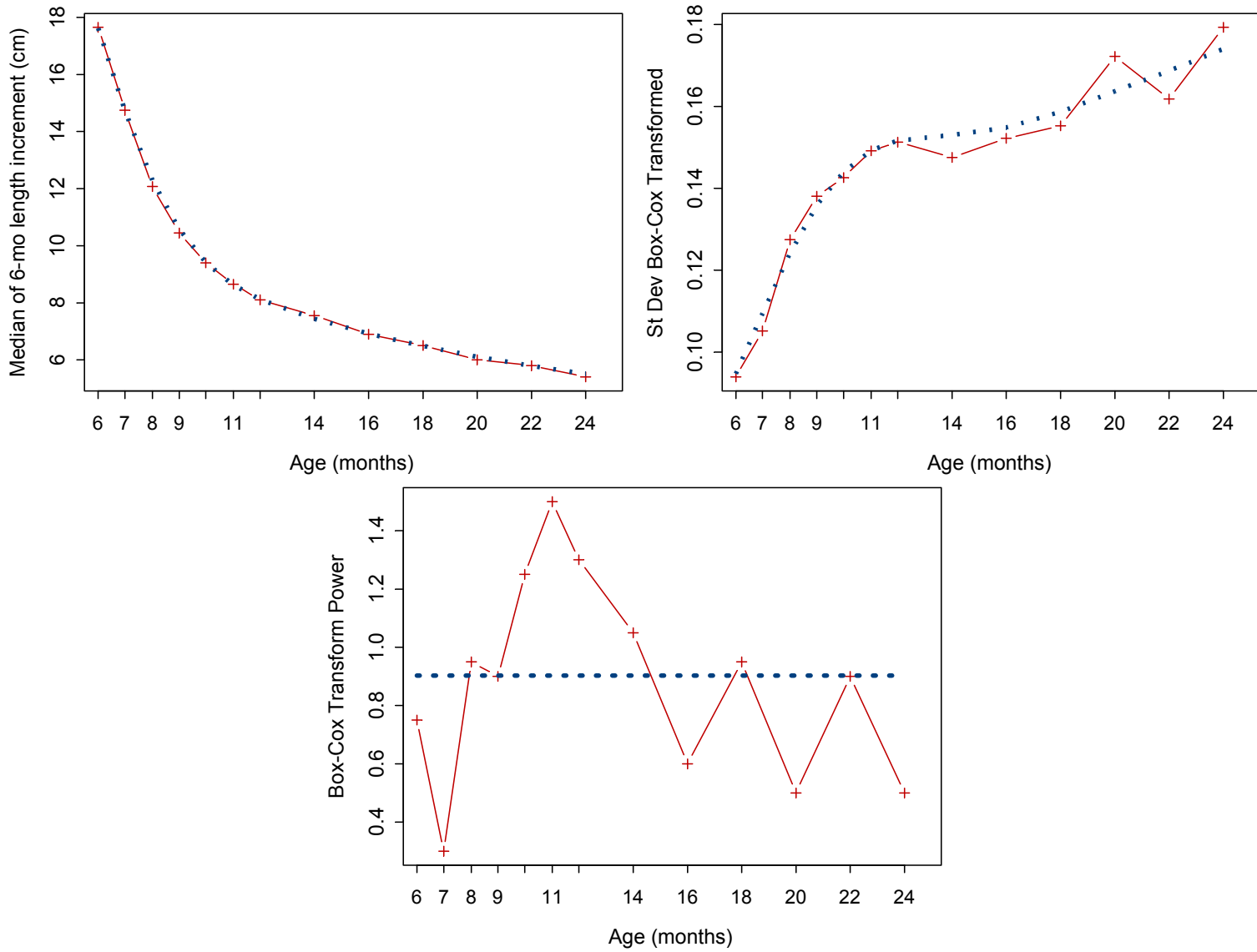
Figure A4. 28 Fitting of the \mu , \sigma , and v curves of selected model for 6-month length velocity for boys
