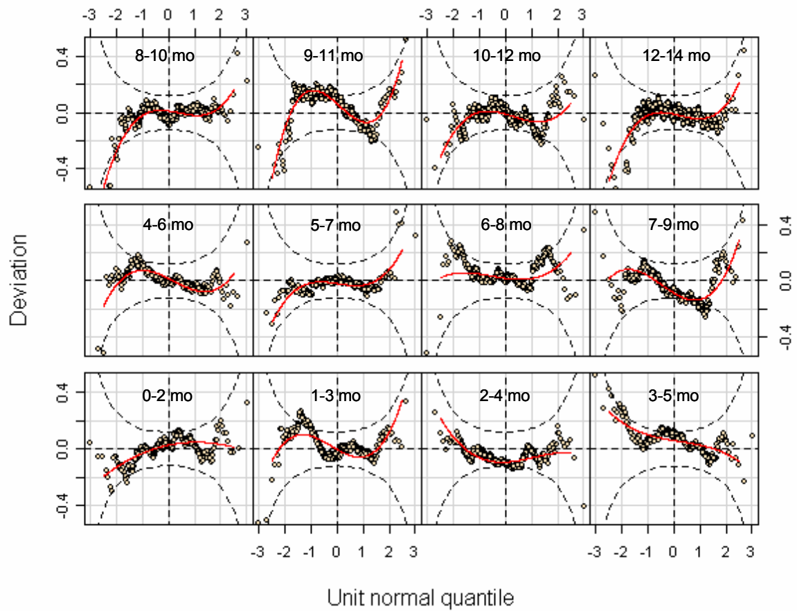
Figure A5.1 Worm plots from selected model [BCPE( x = \text{age}^{0.05} , df(\mu) = 8 , df(\sigma) = 4 , df(\nu) = 4 , \tau = 2 )] for 2-month head circumference velocity for boys
