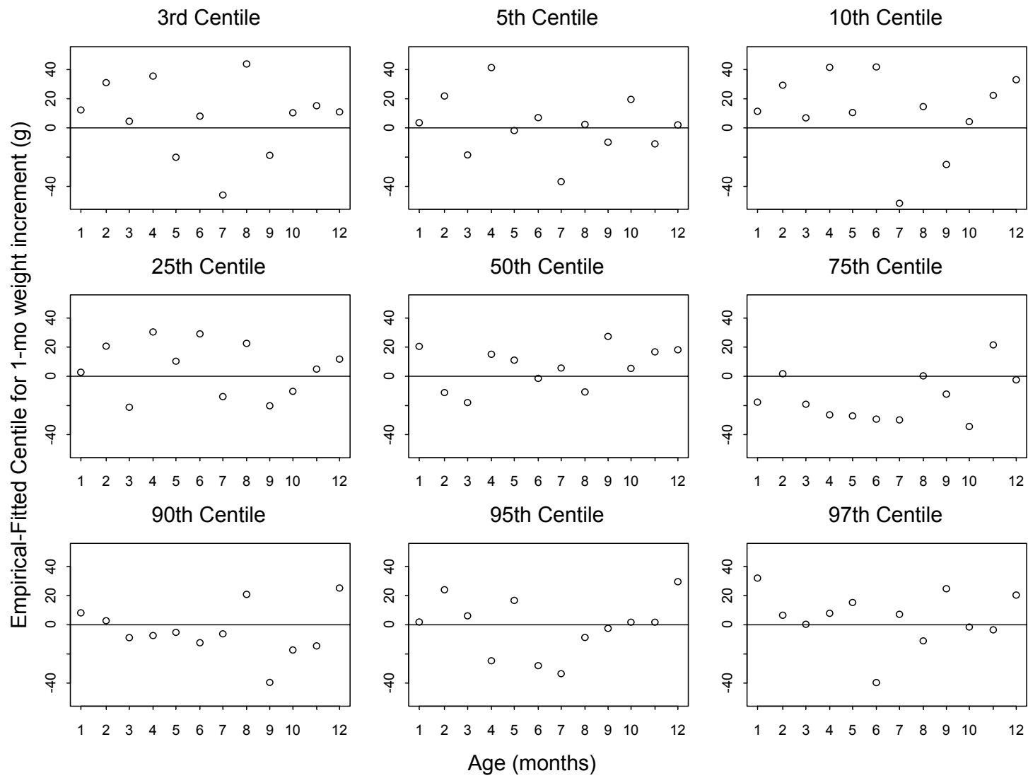
Figure A3.10 Centile residuals from fitting selected model for 1-month weight velocity for girls
