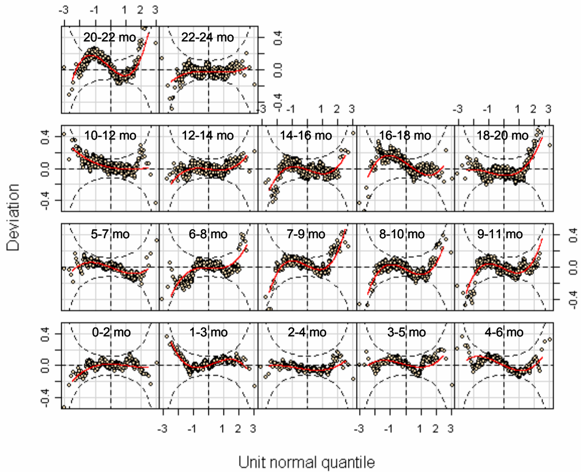
Figure A3.16 Worm plots from selected model [BCPE( x=age^{0.05} , df(\mu)=12 , df(\sigma)=5 , df(\nu)=4 , \tau=2 )] for 2-month weight velocity for girls
