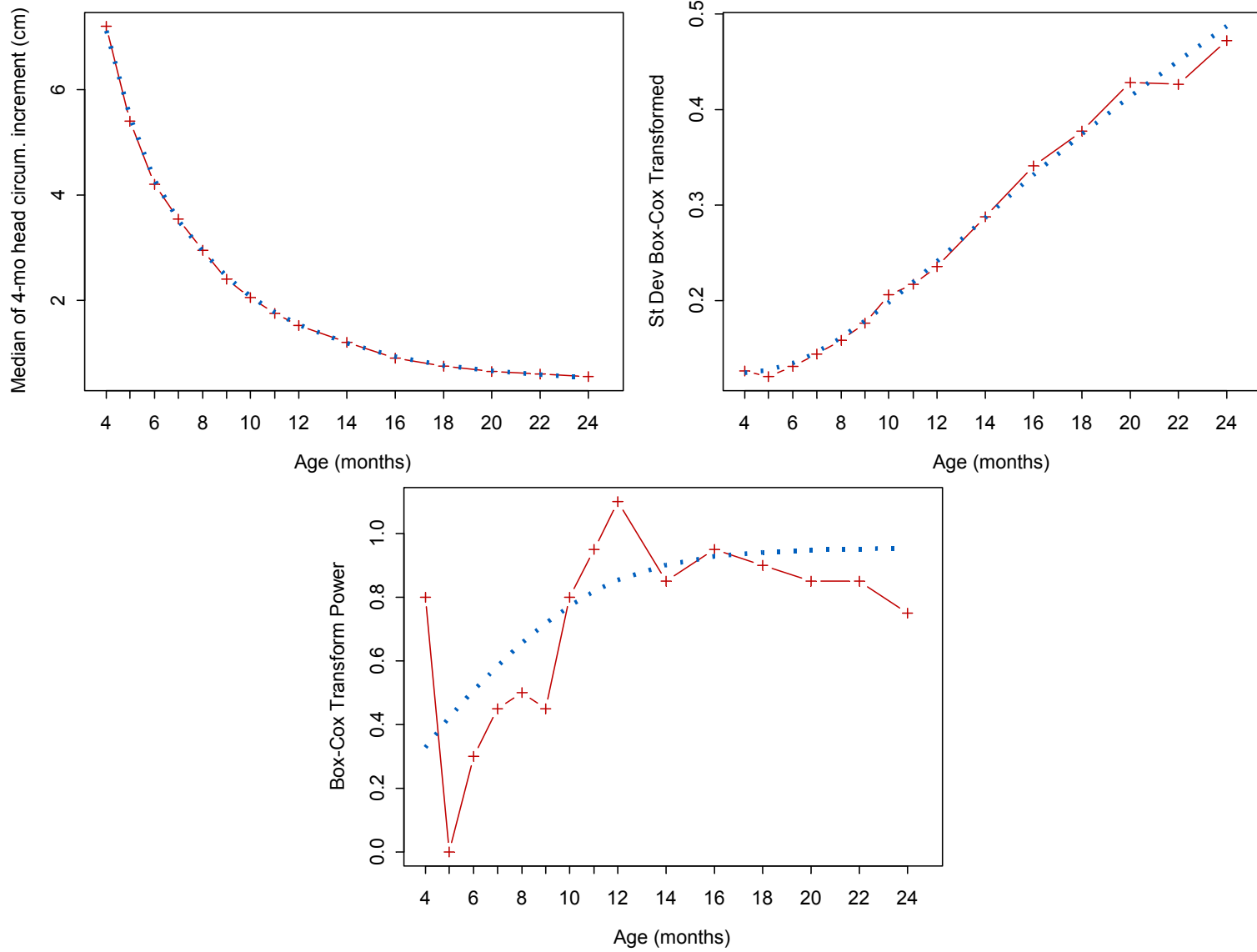
Figure A5.22 Fitting of the \mu , \sigma , and \nu curves of selected model for 4-month head circumference velocity for boys
