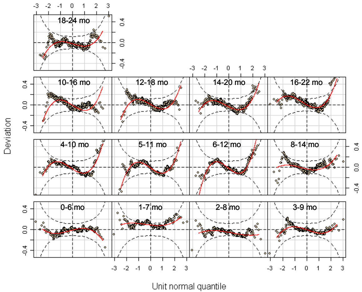
Figure A3.42 Worm plots from selected model [BCPE( x=age^{0.05} , df(\mu)=7 , df(\sigma)=5 , df(v)=4 , \tau=2 )] for 6-month weight velocity for girls
