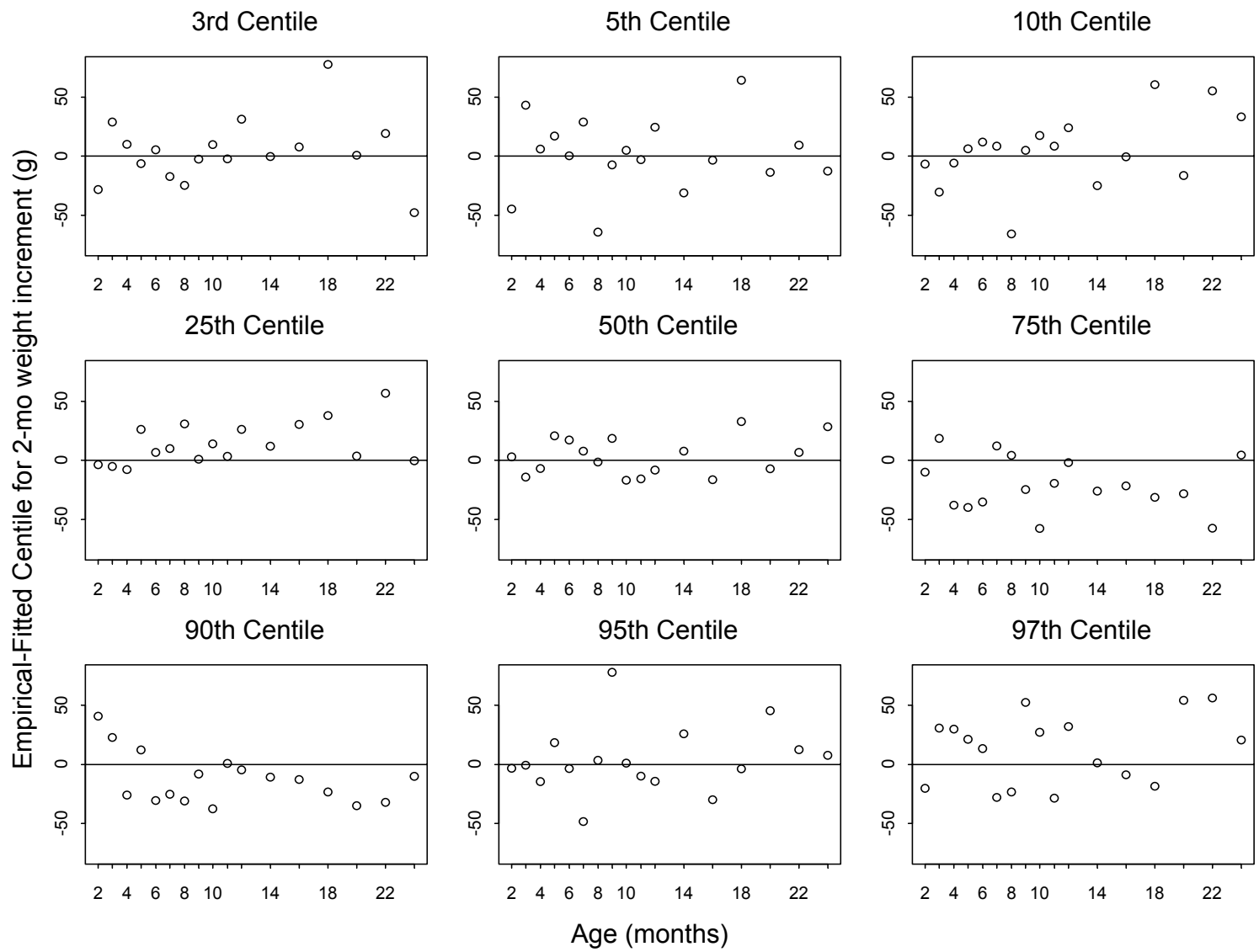
Figure A3.20 Centile residuals from fitting selected model for 2-month weight velocity for girls
