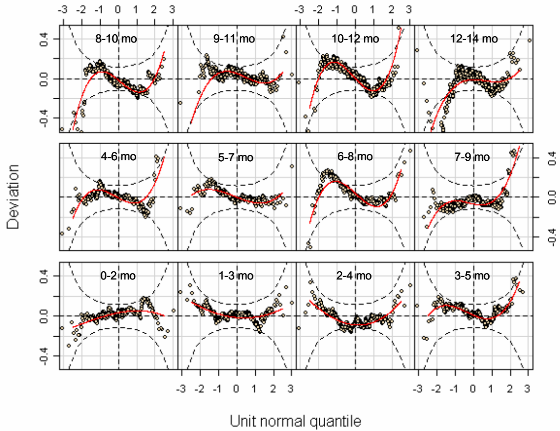
Figure A5.6 Worm plots from selected model [BCPE( x=age^{0.05} , df(\mu)=8 , df(\sigma)=4 , df(v)=1 , \tau=2 )] for 2-month head circumference velocity for girls
