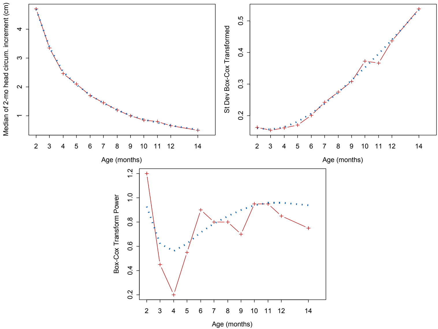
Figure A5.2 Fitting of the \mu , \sigma , and \nu curves of selected model for 2-month head circumference velocity for boys
