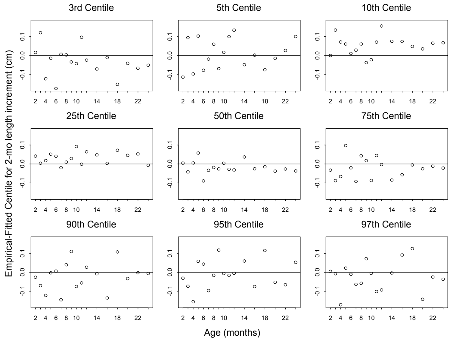
Figure A4.10 Centile residuals from fitting selected model for 2-month length velocity for girls
