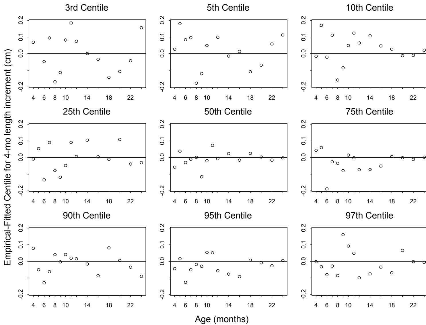
Figure A4.26 Centile residuals from fitting selected model for 4-month length velocity for girls
