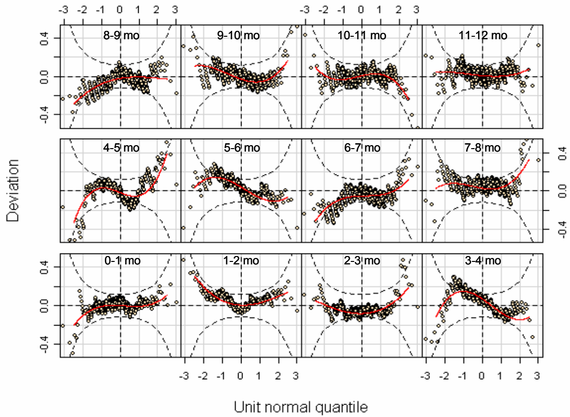
Figure A3.6 Worm plots from selected model [BCPE( x=age^{0.05} , df(\mu)=9 , df(\sigma)=4 , df(v)=1 , \tau=2 )] for 1-month weight velocity for girls
