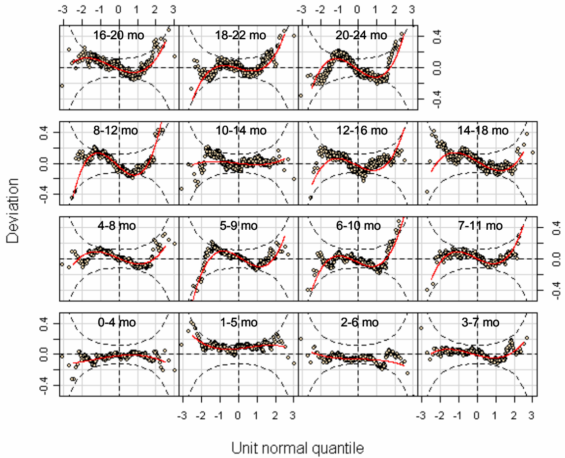
Figure A3.32 Worm plots from selected model [BCPE( x=age^{0.05} , df(\mu)=9 , df(\sigma)=5 , df(v)=5 , \tau=2 )] for 4-month weight velocity for girls
