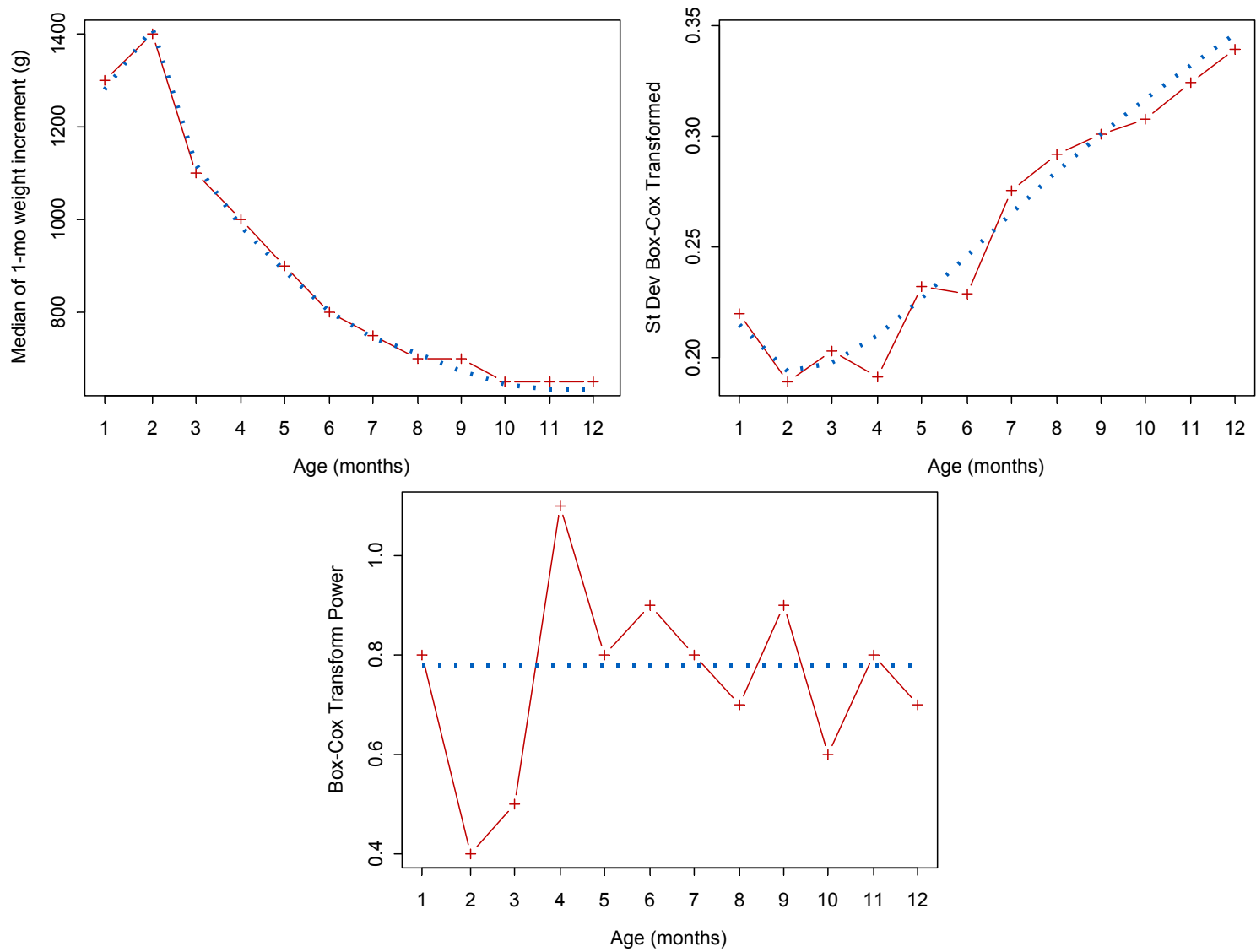
Figure A3.7 Fitting of the \mu , \sigma , and \nu curves of selected model for 1-month weight velocity for girls
