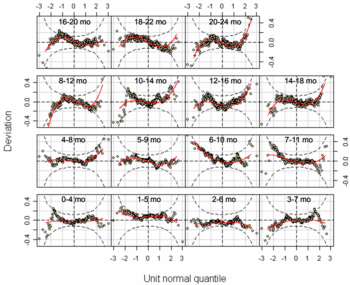
Figure A3.27 Worm plots from selected model [BCPE( x=age^{0.05} , df(\mu)=11 , df(\sigma)=5 , df(v)=5 , \tau=2 )] for 4-month weight velocity for boys
