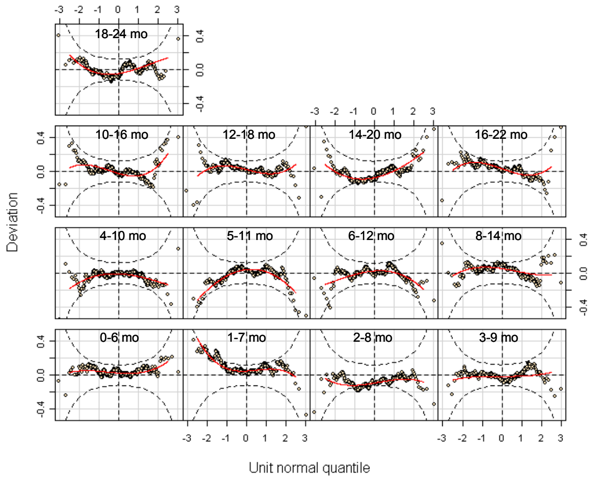
Figure A4.27 Worm plots from selected model [BCPE( x = \text{age}^{0.05} , df(\mu) = 7 , df(\sigma) = 5 , df(v) = 1 , \tau = 2 )] for 6-month length velocity for boys
