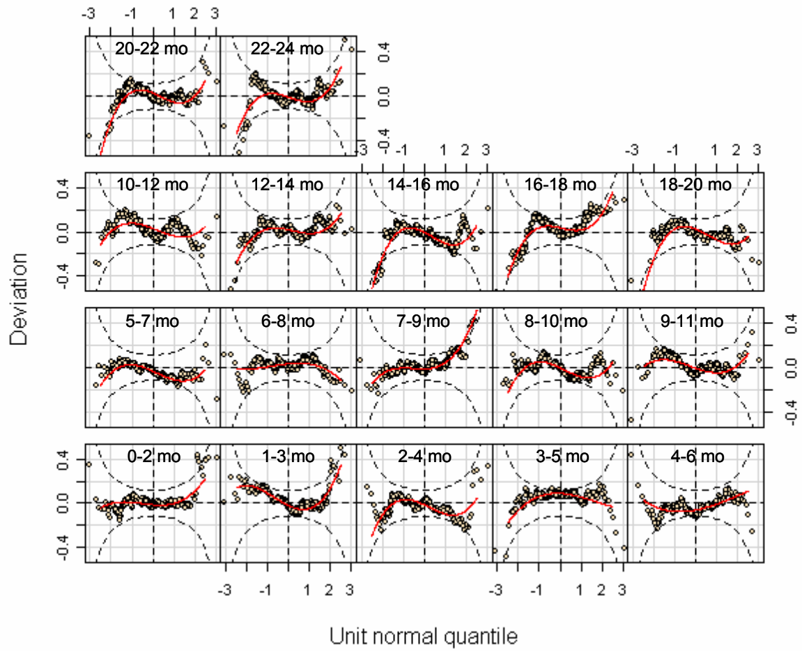
Figure A4.6 Worm plots from selected model [BCPE( x=\text{age}^{0.05} , df(\mu)=10 , df(\sigma)=7 , df(v)=1 , \tau=2 )] for 2-month length velocity for girls
