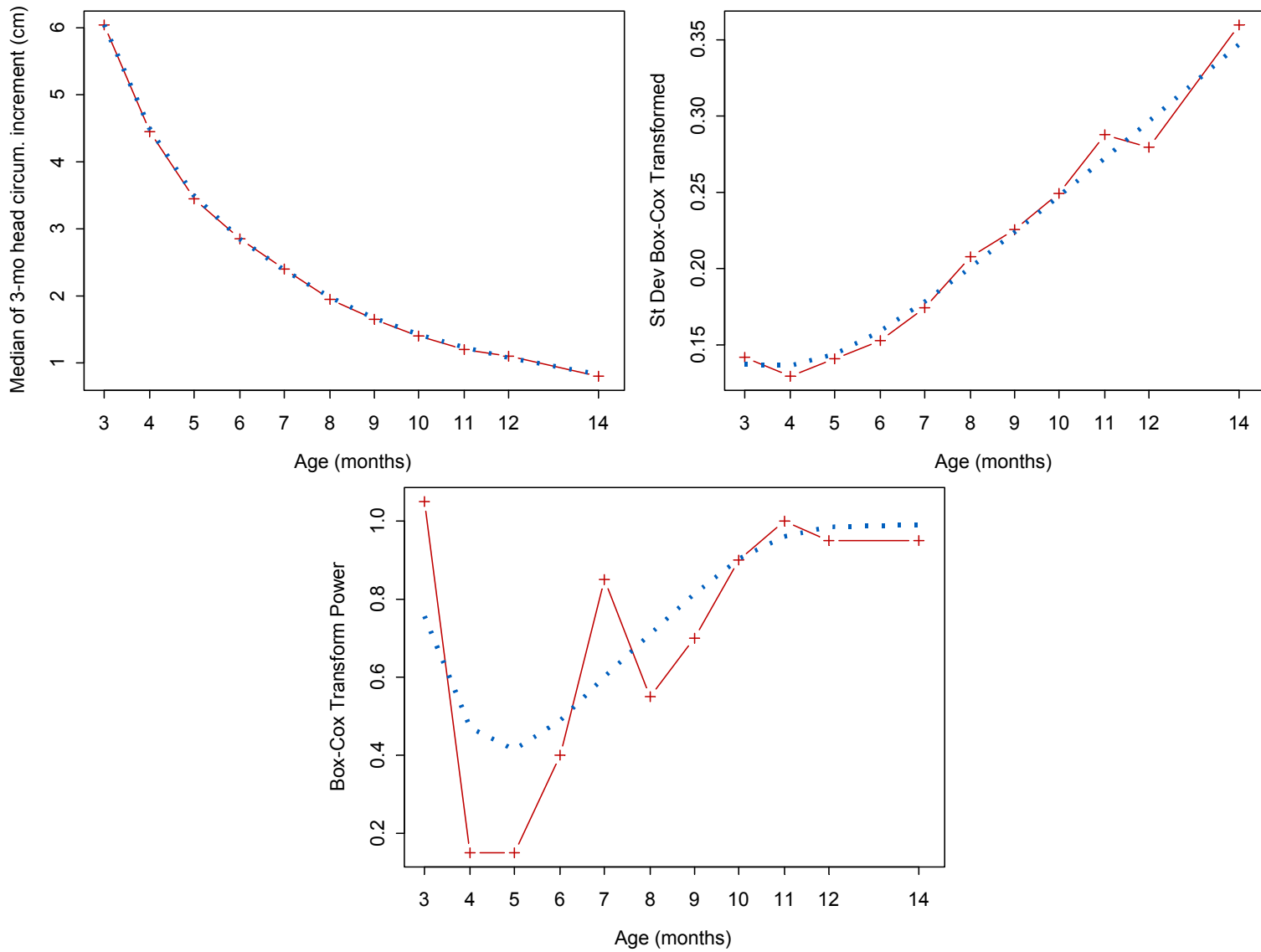
Figure A5.12 Fitting of the \mu , \sigma , and \nu curves of selected model for 3-month head circumference velocity for boys
