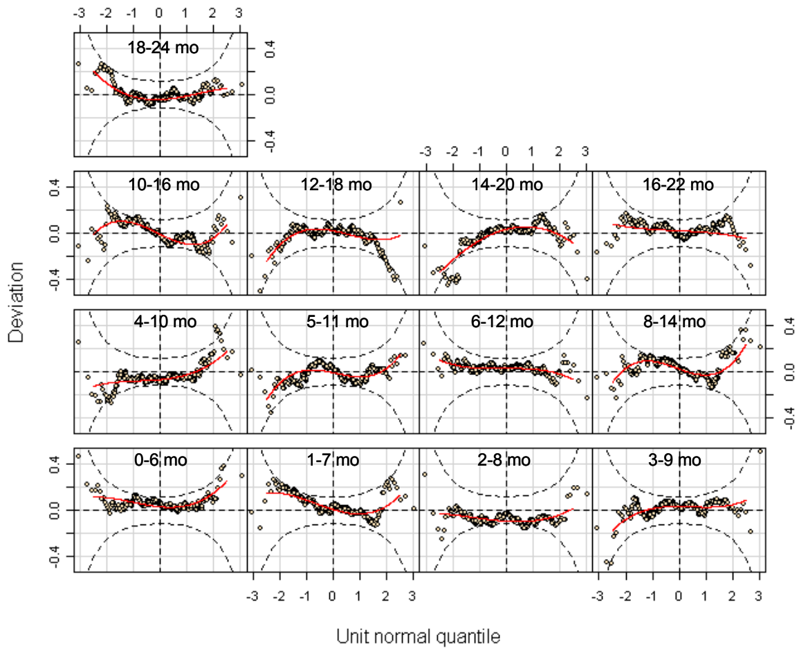
Figure A4.32 Worm plots from selected model [BCPE( x = \text{age}^{0.05} , df(\mu) = 7 , df(\sigma) = 4 , df(\nu) = 1 , \tau = 2 )] for 6-month length velocity for girls
