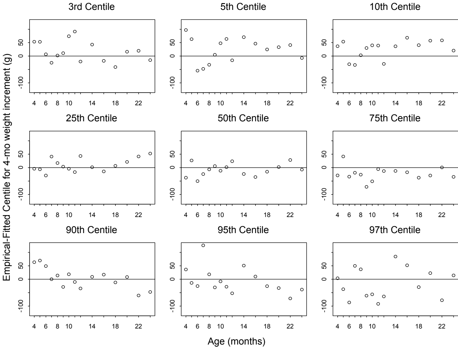
Figure A3.31 Centile residuals from fitting selected model for 4-month weight velocity for boys
