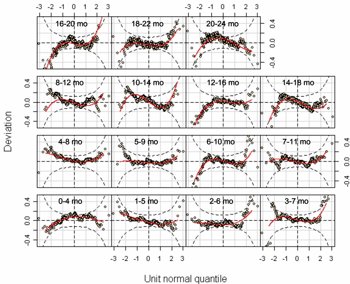
Figure A5.26 Worm plots from selected model [BCPE( x=age^{0.05} , df(\mu)=10 , df(\sigma)=5 , df(\nu)=2 , \tau=2 )] for 4-month head circumference velocity for girls
