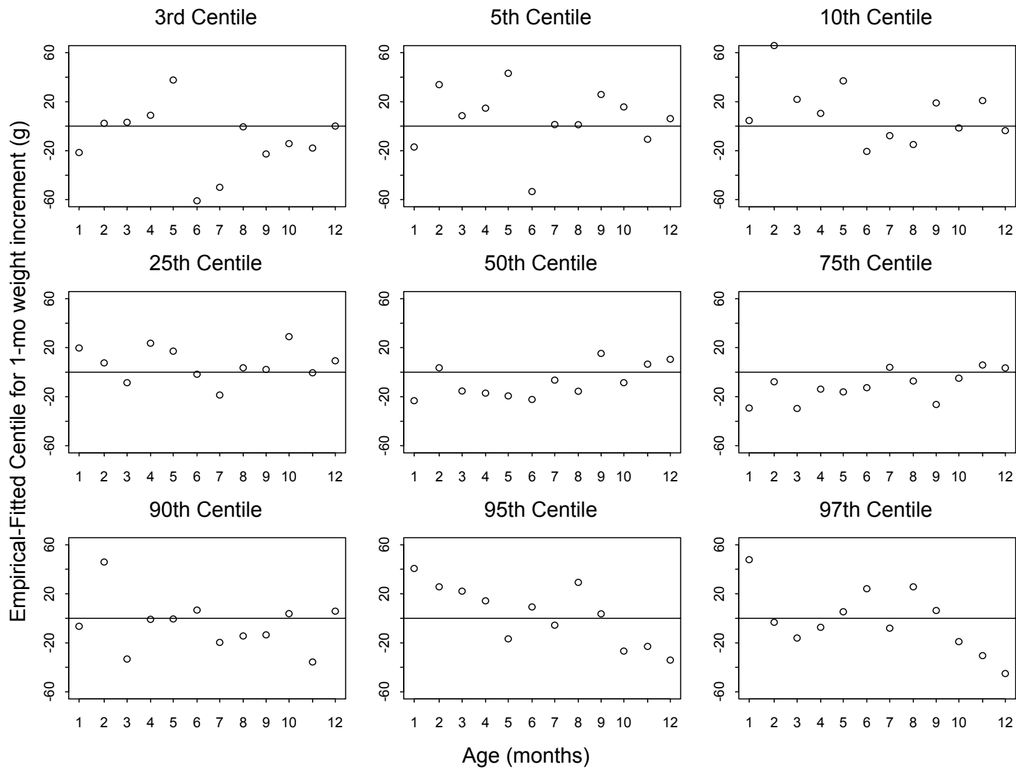
Figure A3.5 Centile residuals from fitting selected model for 1-month weight velocity for boys
