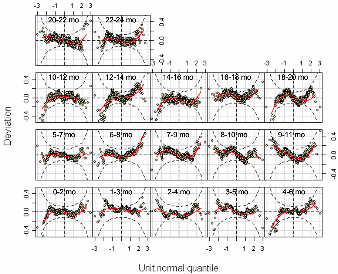
Figure A3.11 Worm plots from selected model [BCPE( x=\text{age}^{0.05} , df(\mu)=12 , df(\sigma)=6 , df(\nu)=3 , \tau=2 )] for 2-month weight velocity for boys
