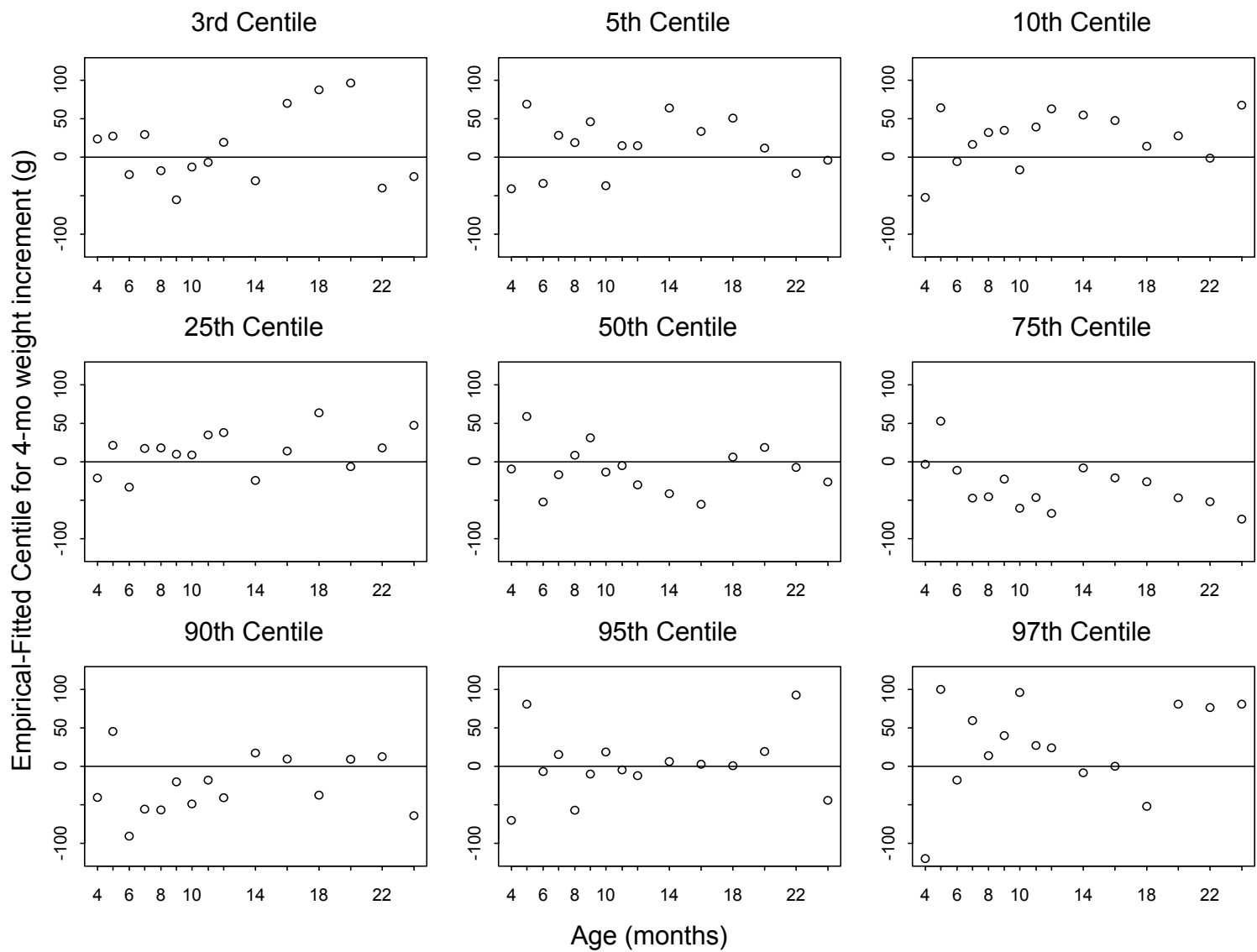
Figure A3.36 Centile residuals from fitting selected model for 4-month weight velocity for girls
