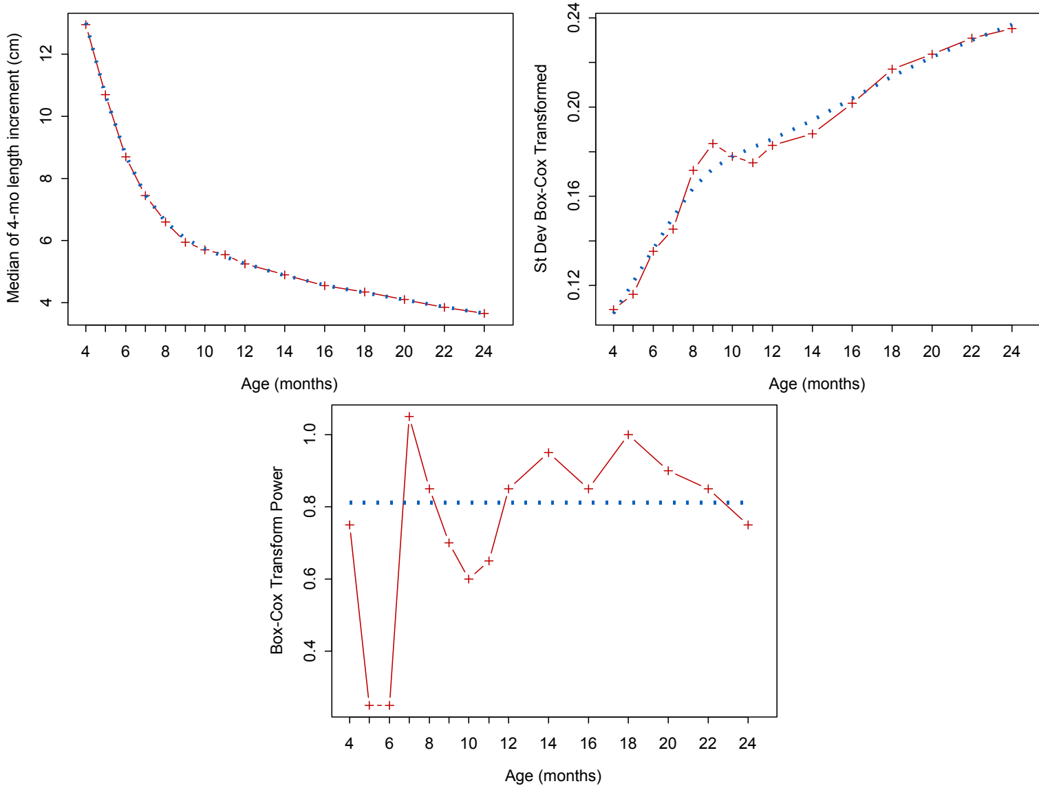
Figure A4.23 Fitting of the \mu , \sigma , and \nu curves of selected model for 4-month length velocity for girls
